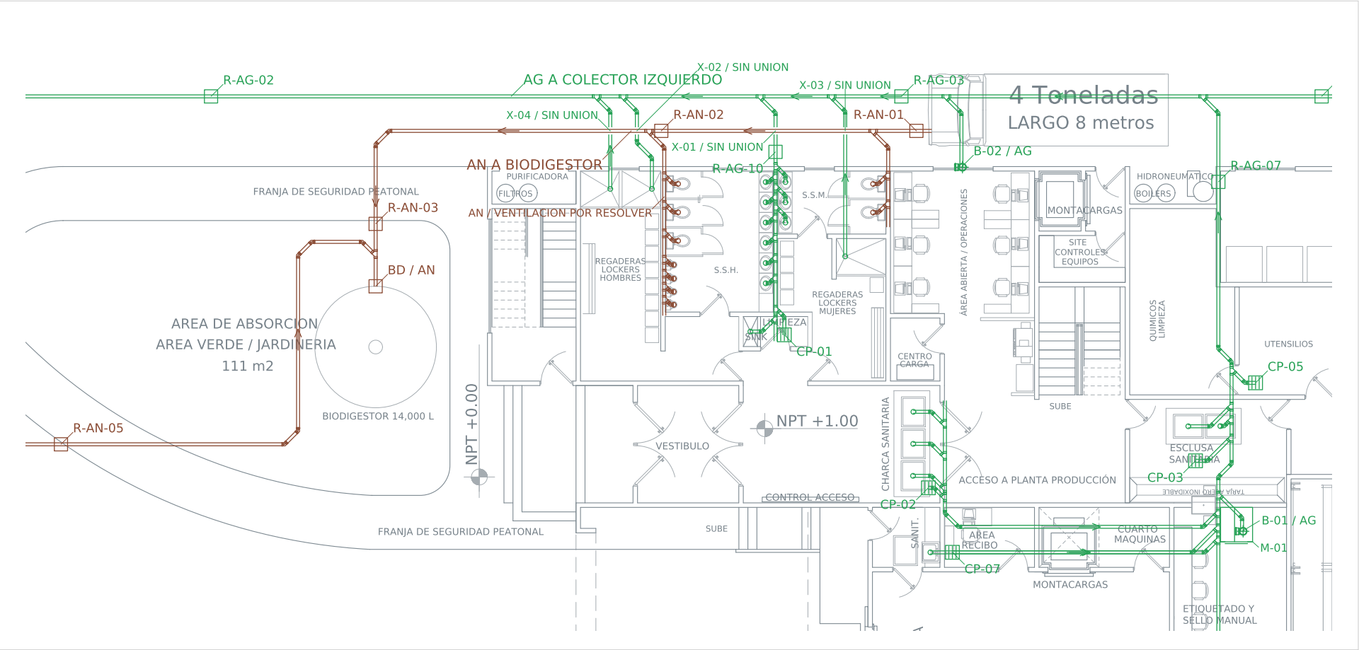
AG / AN · Changing facilities and sanitary filters
