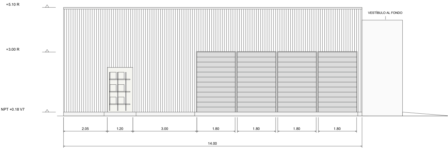
South facade · architectural elevation
