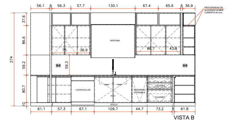
02 / Sink wall and upper cabinetry
