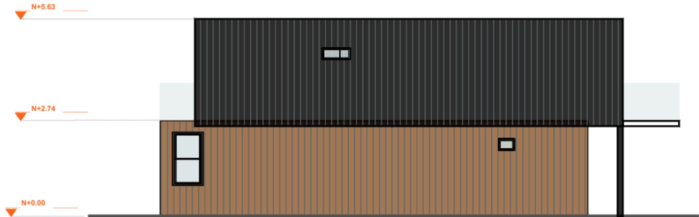
LEFT ELEVATION
